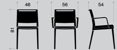
4-legged chair Silla 4 patas Chaise 4 pieds
