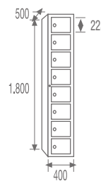
STV8-40/1 COD. 44081
