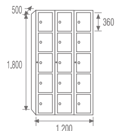
STV5-40/3 COD. 44053
