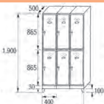
ST-40/3 COD. 44013
